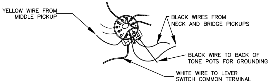
S-1 SWITCH WIRING DETAIL
